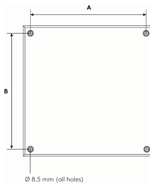
Figure 1. Mounting Diagram.
