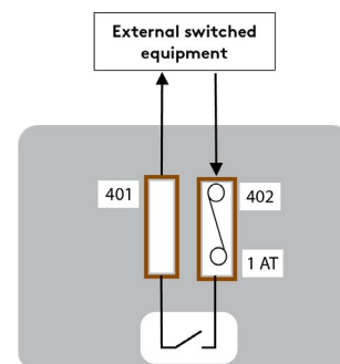
Figure 7. Output Wiring
