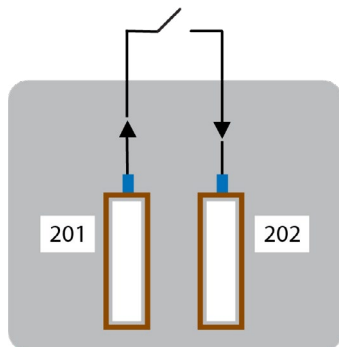
Figure 6. Input Wiring
