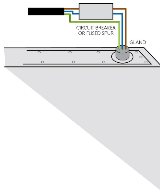
Figure 2. Mains Supply Feed.
